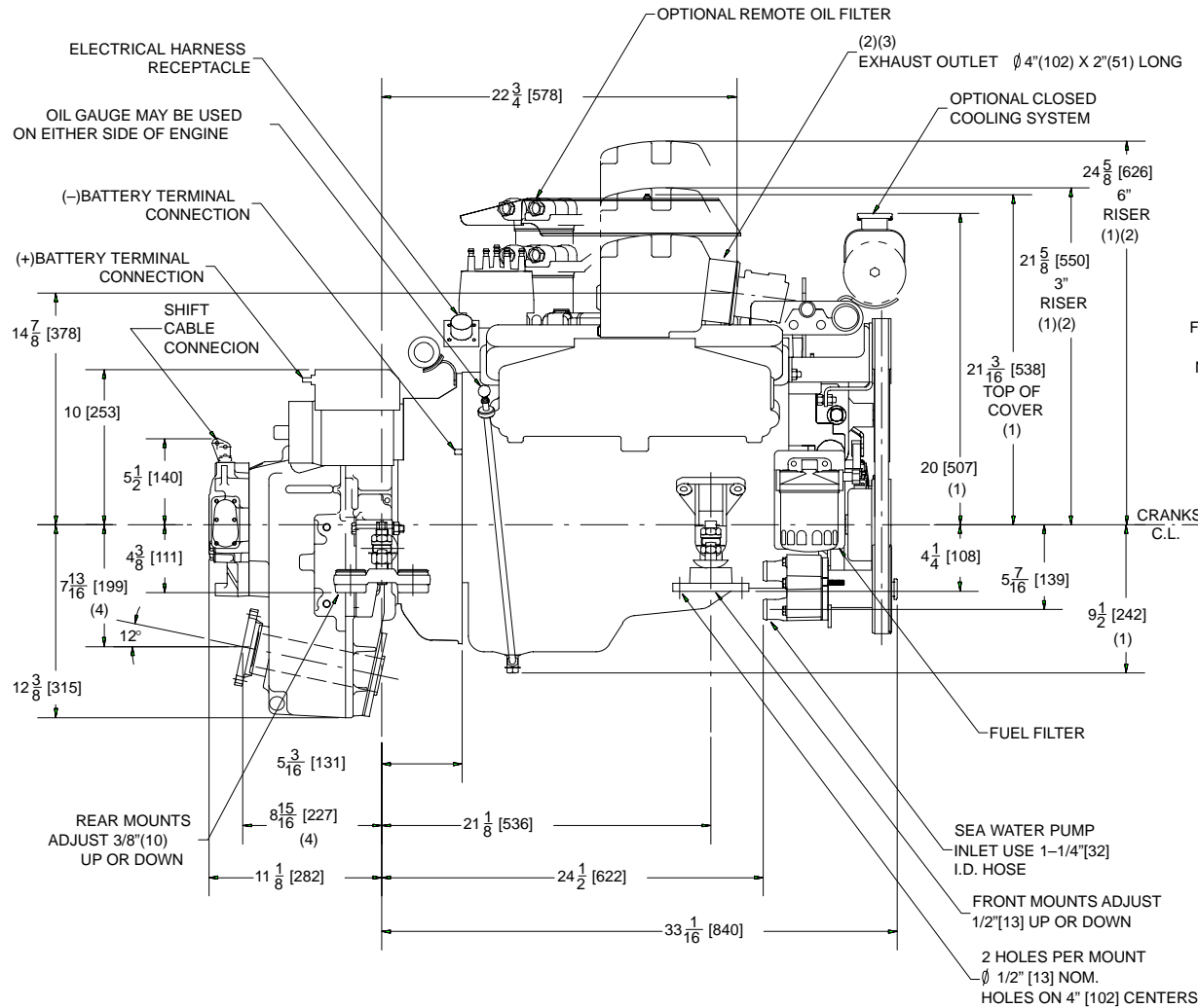
MIE 5.7L WITH VELVET DRIVE 5000A DOWN ANGLE TRANSMISSION
