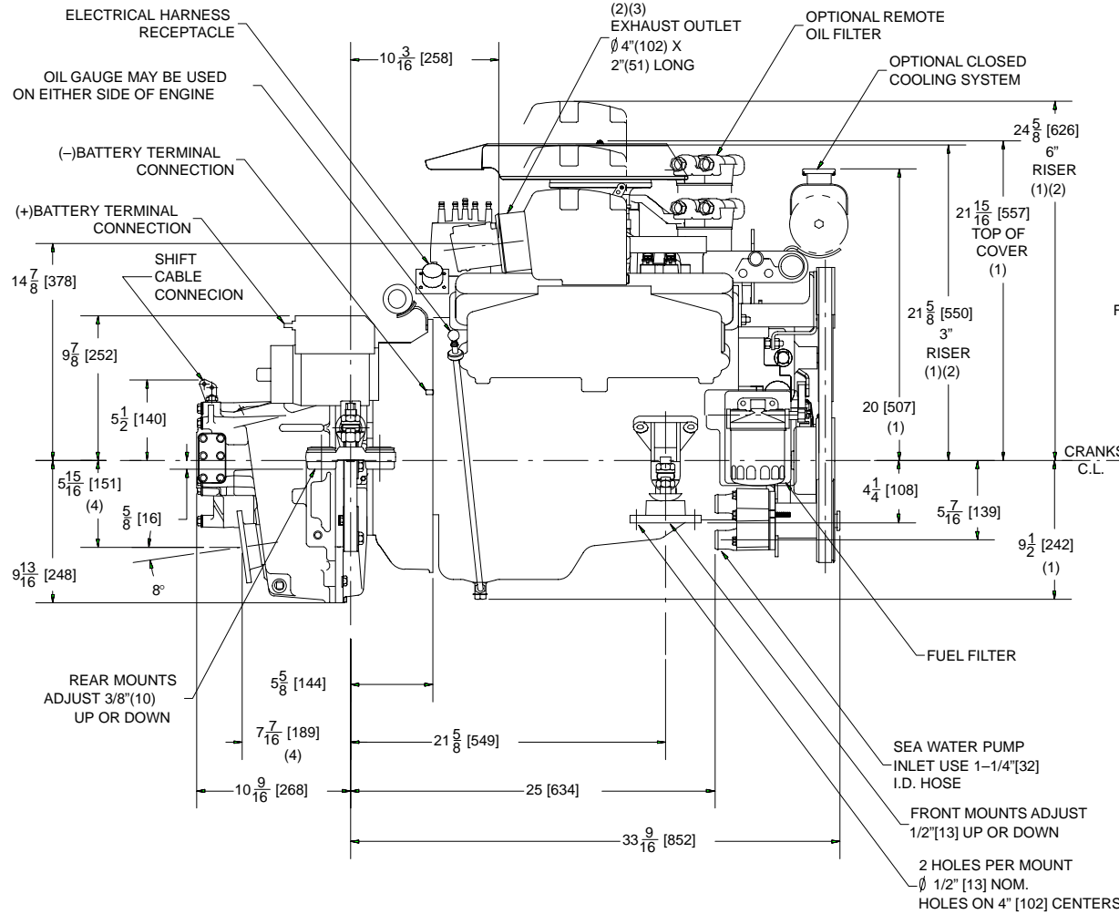
MIE 350 MAG MPI WITH VELVET DRIVE 5000A DOWN ANGLE TRANSMISSION
