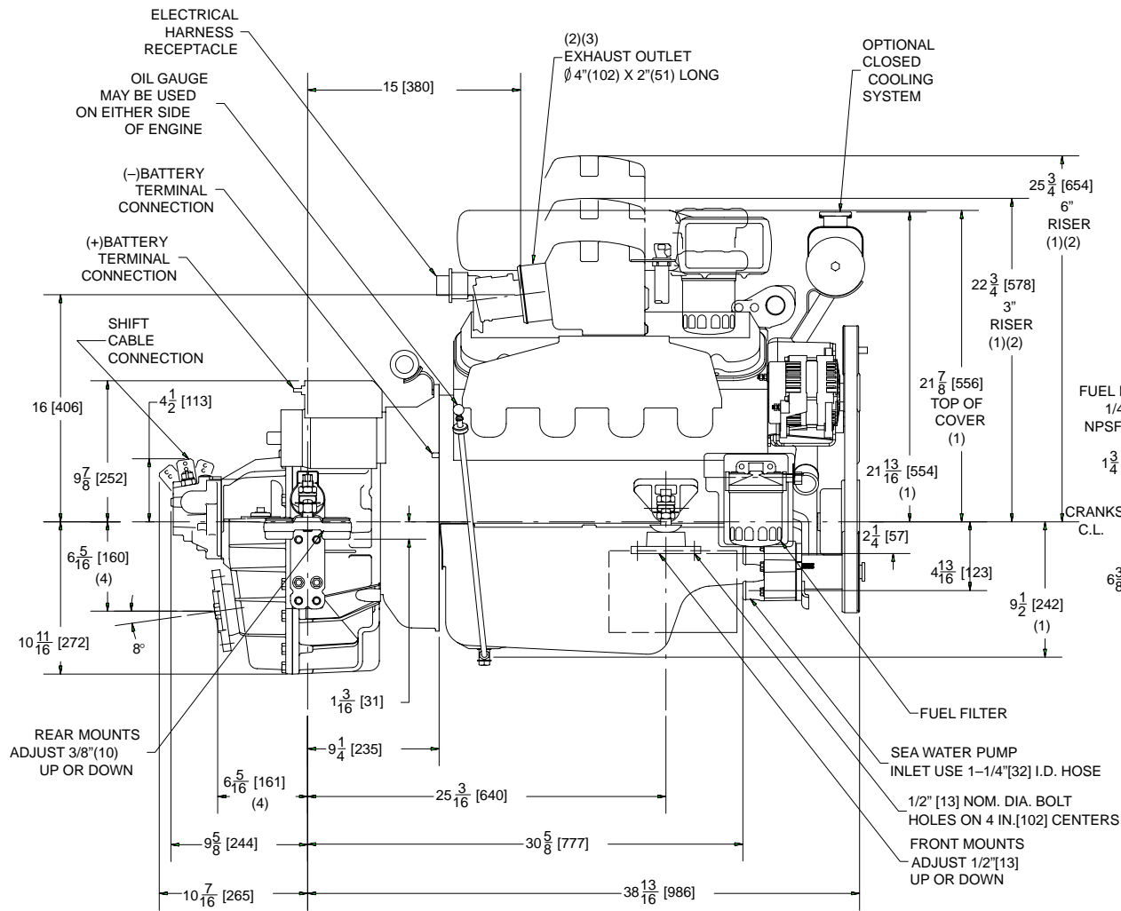
MIE 8.2L MPI WITH HURTH 800A DOWN ANGLE TRANSMISSION
