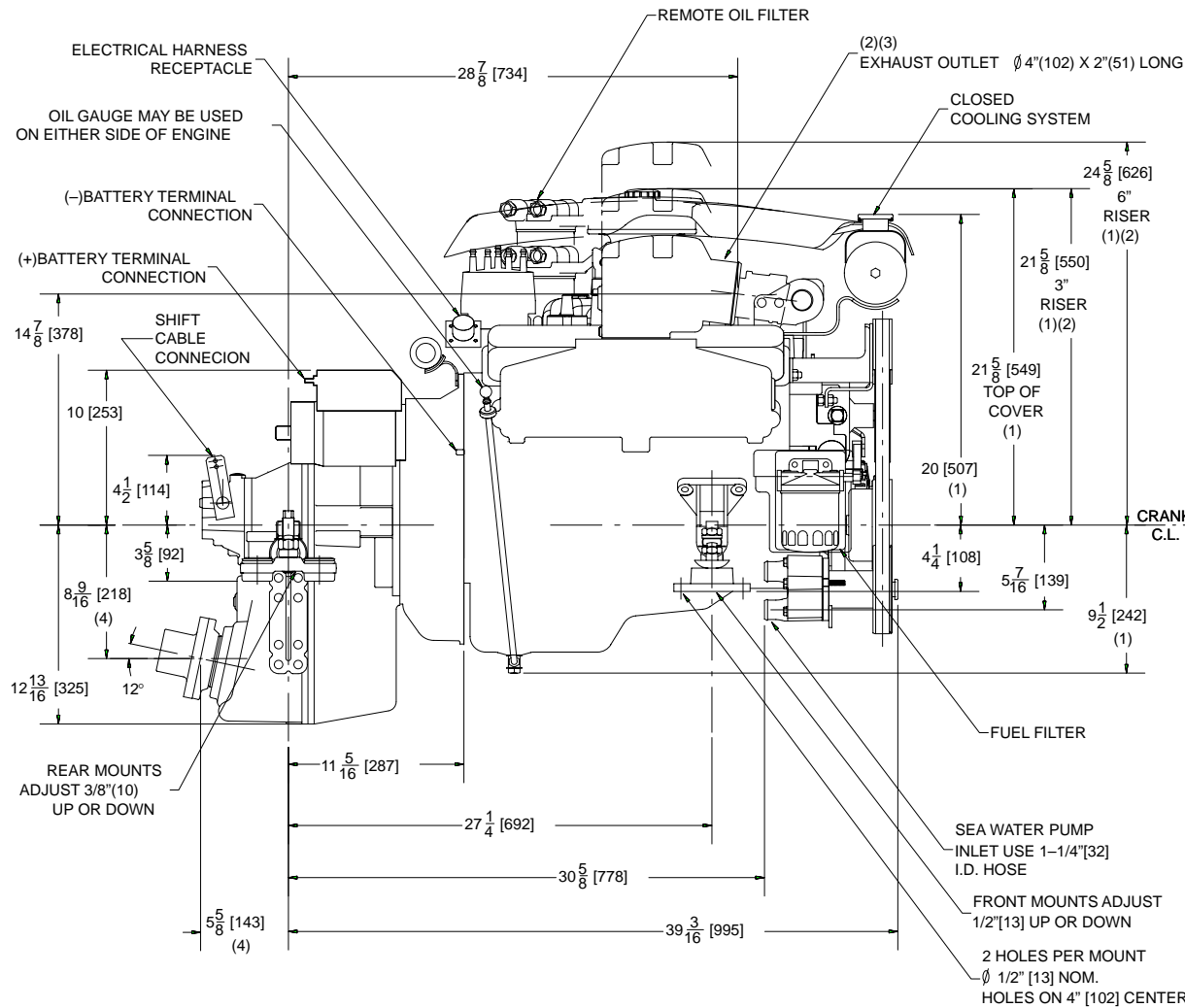
MIE 350 MAG MPI HORIZON WITH HURTH 630V V-DRIVE TRANSMISSION
