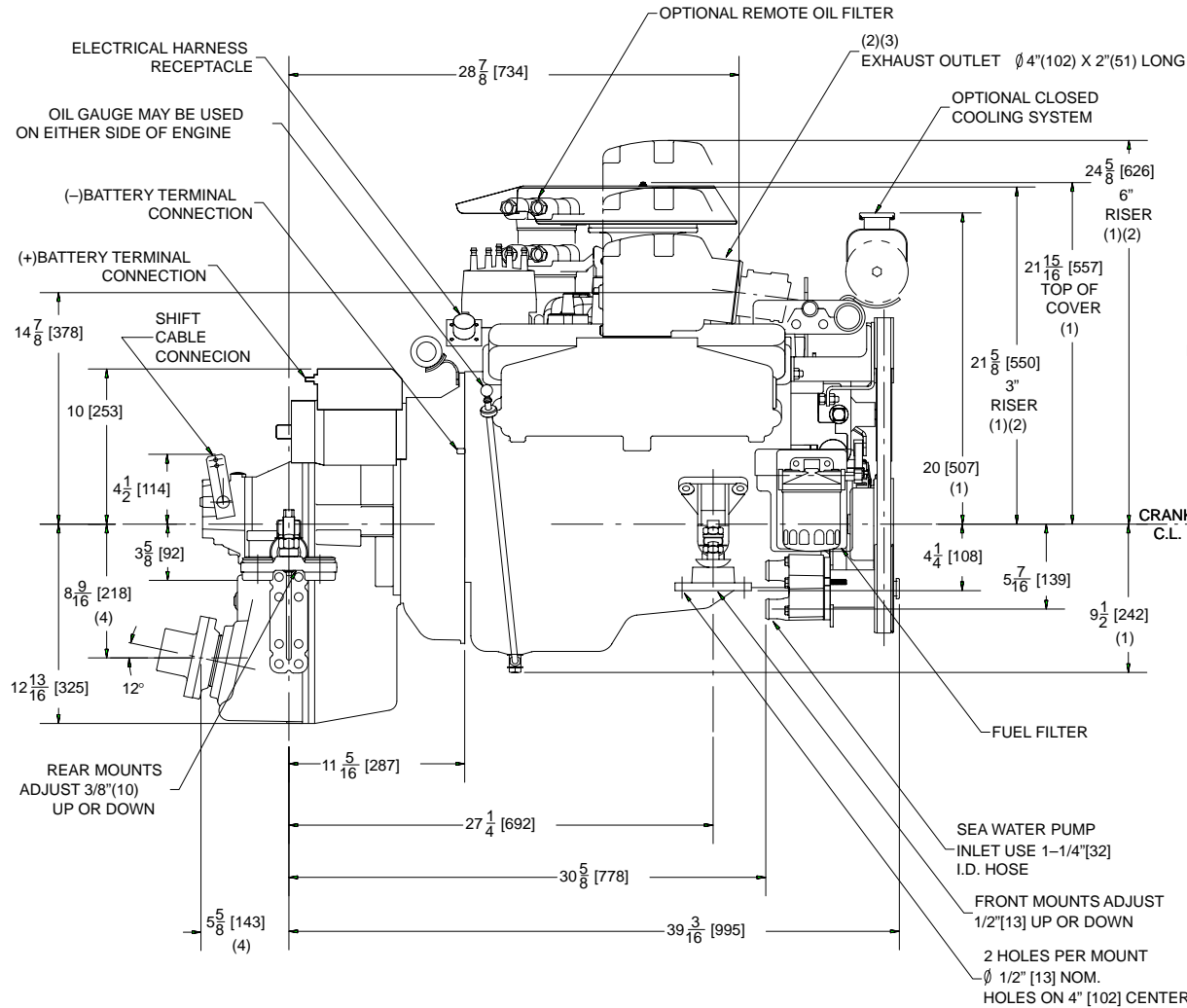
MIE 350 MAG MPI WITH HURTH 630V V-DRIVE TRANSMISSION
