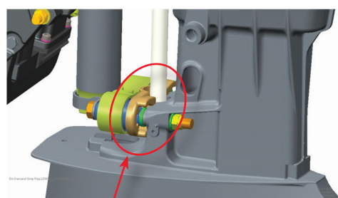
New lower mount snubber and hard washer
