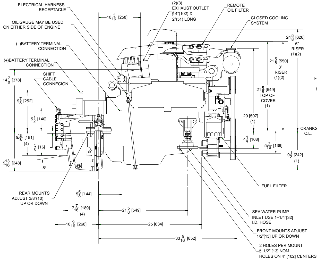
MIE 350 MAG MPI HORIZON WITH VELVET DRIVE 5000A DOWN ANGLE TRANSMISSION
