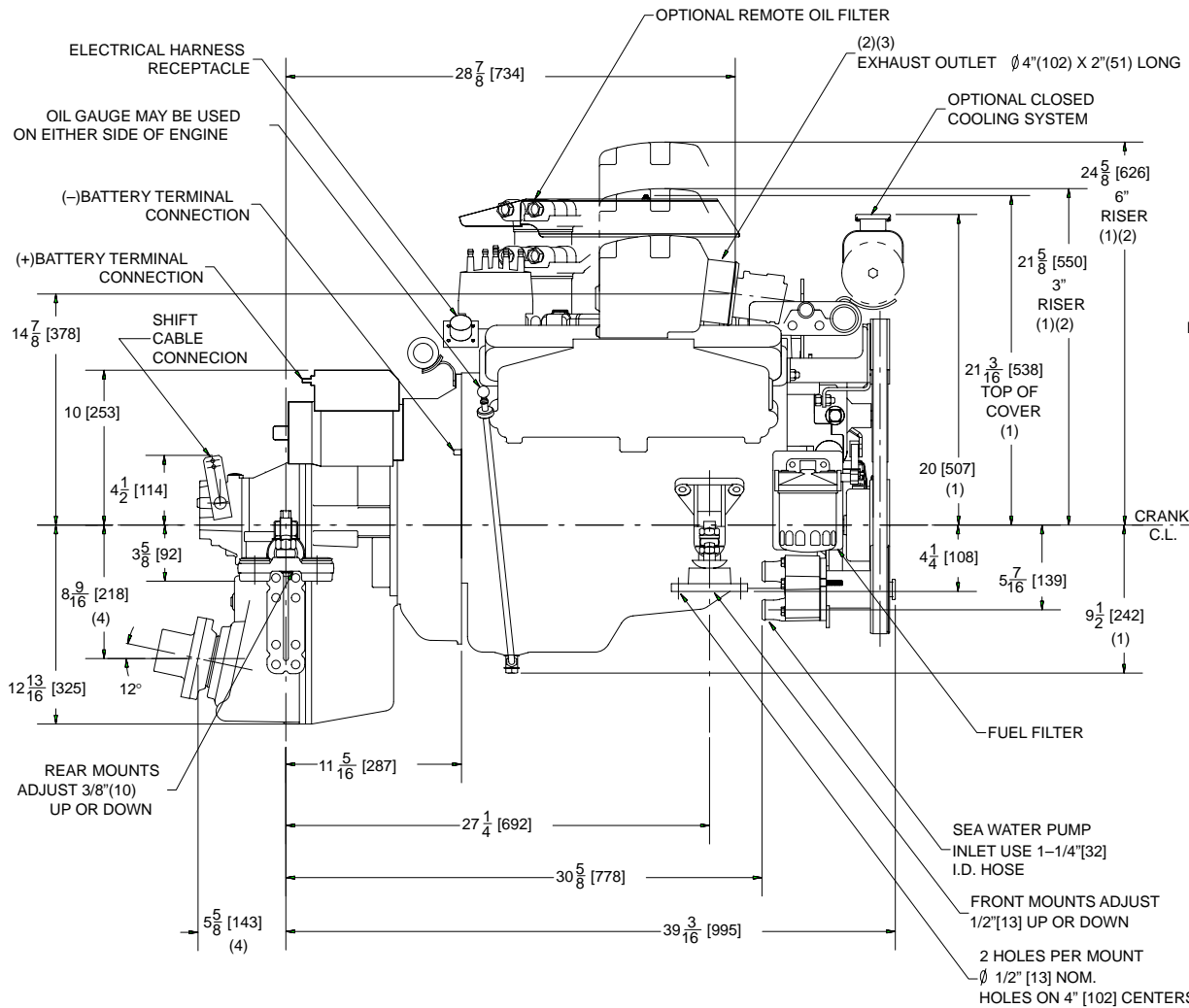
MIE 5.7L WITH HURTH 630V V-DRIVE TRANSMISSION
