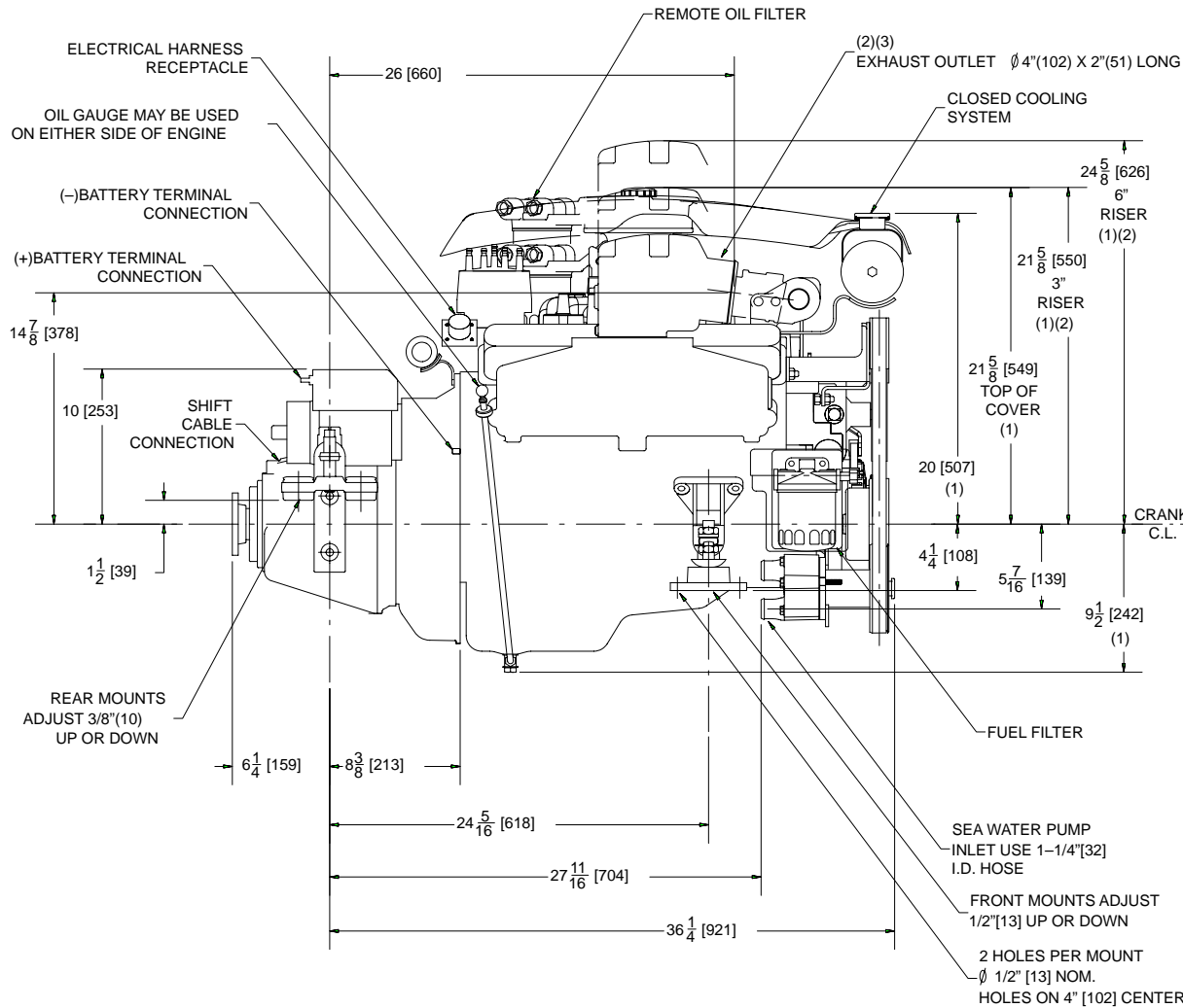
MIE 350 MAG MPI HORIZON WITH VELVET DRIVE 71C REMOTE V-DRIVE TRANSMISSION
